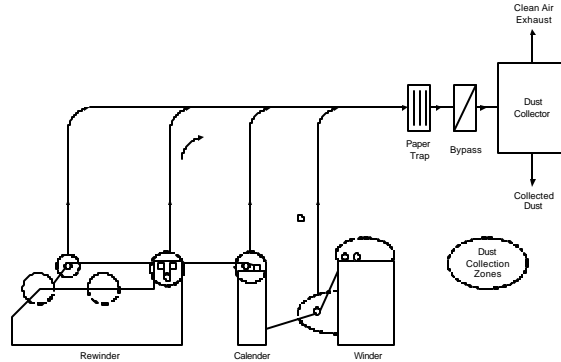
Typical dust collection system layout for a rewriter.
