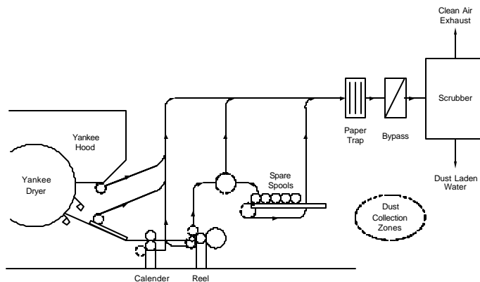
Typical dust collection system layout for a tissue machine.
